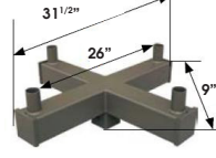
S4VT4S90BZ (4" square pole) S5VT4S90BZ (5" square pole)
